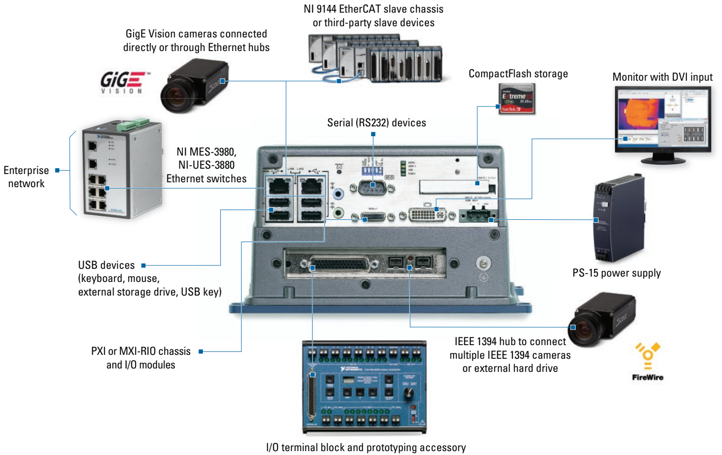
Figure 4. EVS-1464RT and optional accessories
