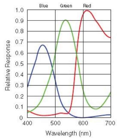
Figure 4. 1774C SXGA Sensor Spectral Response Curves
